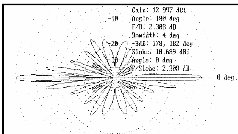
Figure 4: A typical vertical antenna pattern for a 4-element dipole array at about 100 MHz.(VHF), Units in dB. Side-lobes have elevation angles of 72, 57, 15, 40,
